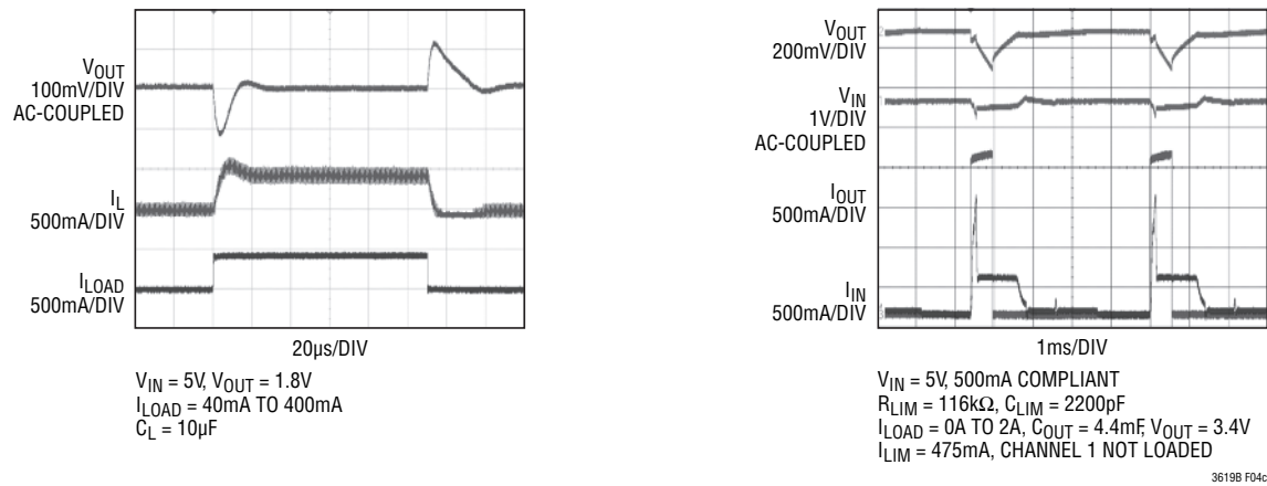
Figure 4c. Transient Response
