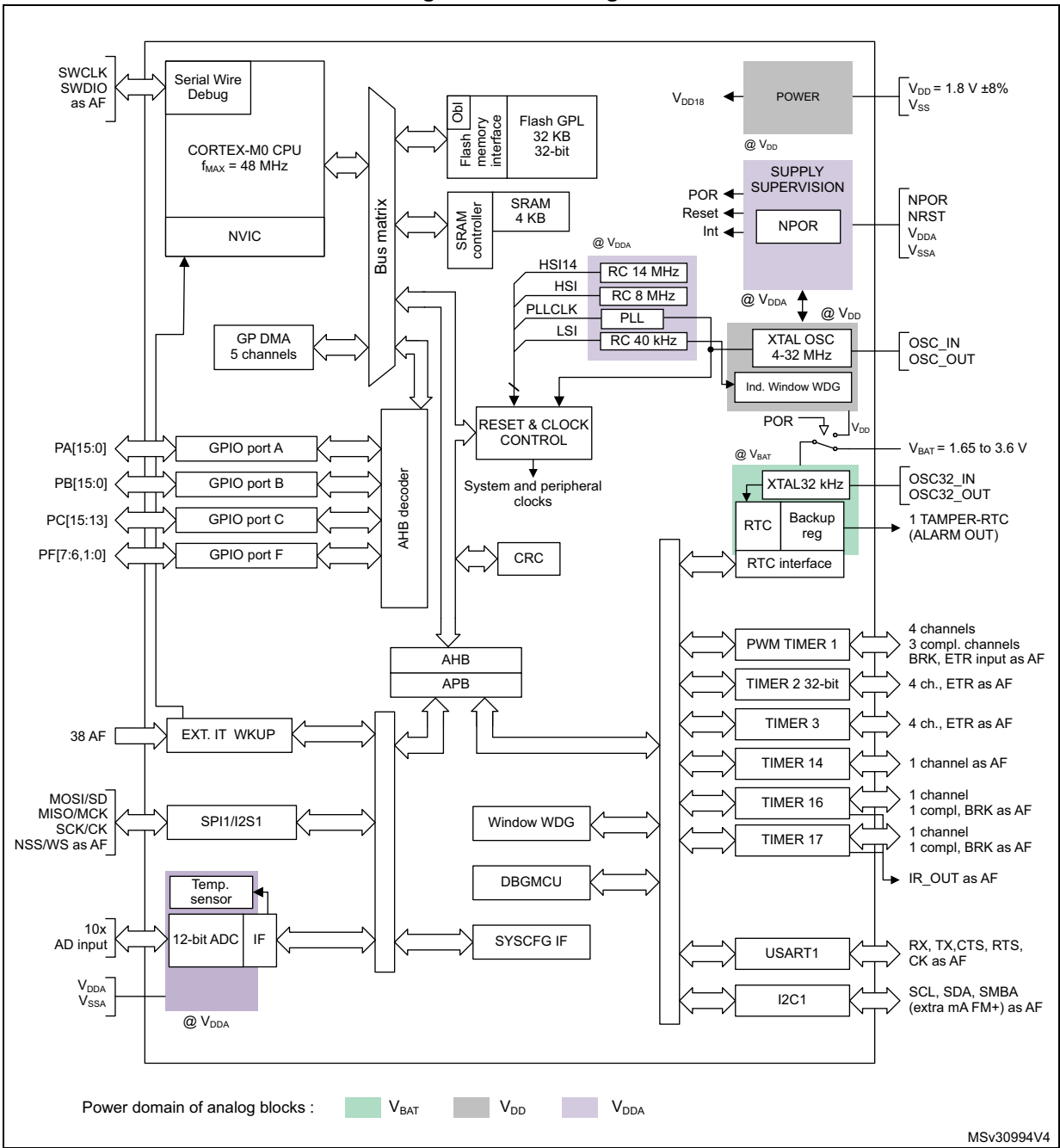
Figure 1. Block diagram
