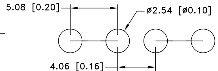
MOUNTING DETAIL FOR 2 CLIPS
