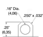
S 5 Solder Eye, extra large & quick connect
