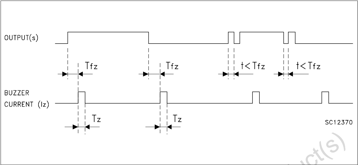
FIGURE 3: Buzzer Functionality
