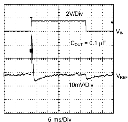
Line Transient Response V_{\text{IN}} = 4\text{V} to 5.5\text{V}
