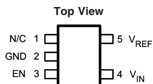
SOT23-5 Package NS Package Number MF05A
