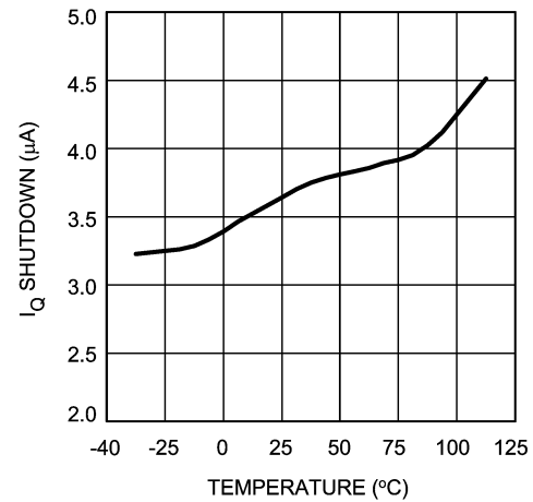
Shutdown I_Q vs Temperature
