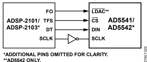
Figure 31. AD5541/AD5542 to ADSP-2101/ADSP-2103 Interface
