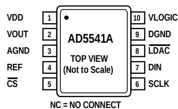
Figure 8. AD5541A 10-Lead MSOP Pin Configuration
