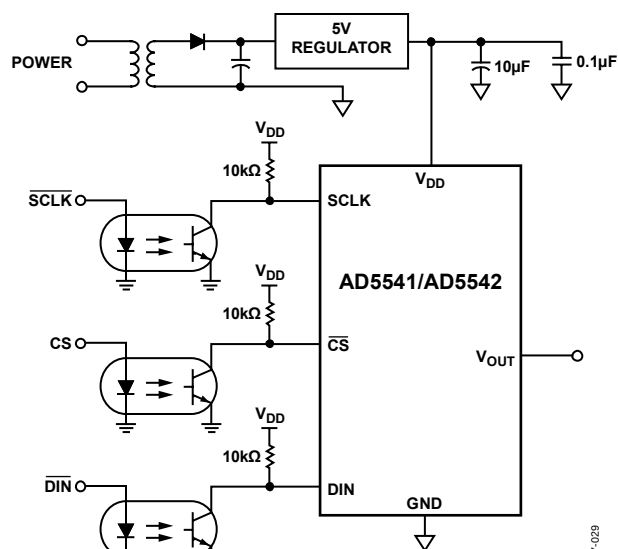
Figure 35. AD5541/AD5542 in an Optocoupler Interface
