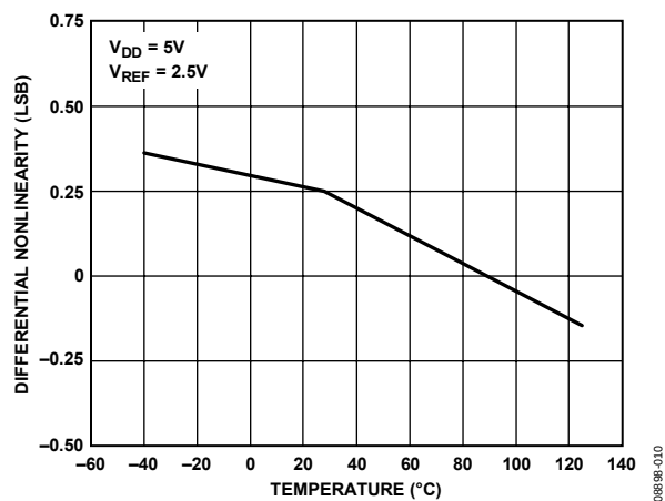
Figure 16. Differential Nonlinearity vs. Temperature
