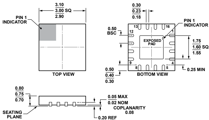
Figure 41. 16-Lead Lead Frame Chip Scale Package [LFCSP]
