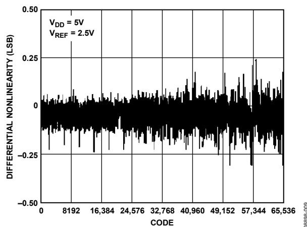
Figure 15. Differential Nonlinearity vs. Code
