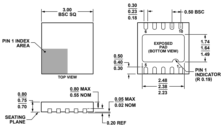
Figure 38. 10-Lead Lead Frame Chip Scale Package [LFCSP] (CP-10-9) Dimensions shown in millimeters.
