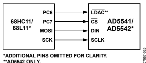
Figure 32. AD5541/AD5542 to 68HC11/68L11 Interface
