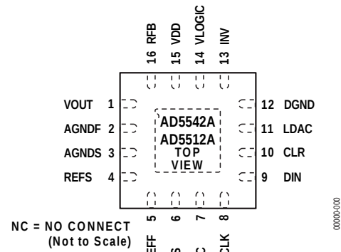
Figure 11. AD5542A 16-Lead LFCSP Pin Configuration
