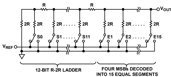
Figure 28. DAC Architecture
