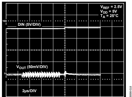
Figure 24. Digital Feedthrough
