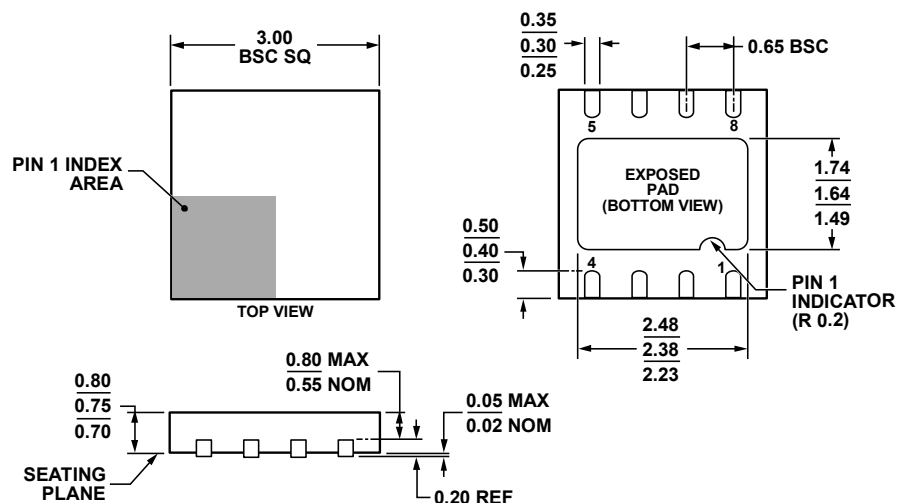
Figure 39. 8-Lead Lead Frame Chip Scale Package [LFCSP]
