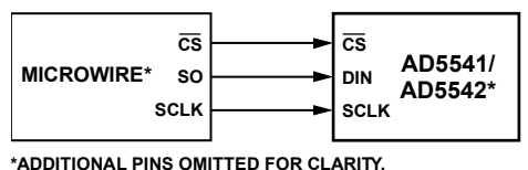
Figure 33. AD5541/AD5542 to MICROWIRE Interface
