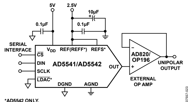
Figure 29. Unipolar Output
