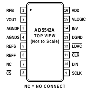
Figure 10. AD5542A 16-Lead TSSOP Pin Configuration
