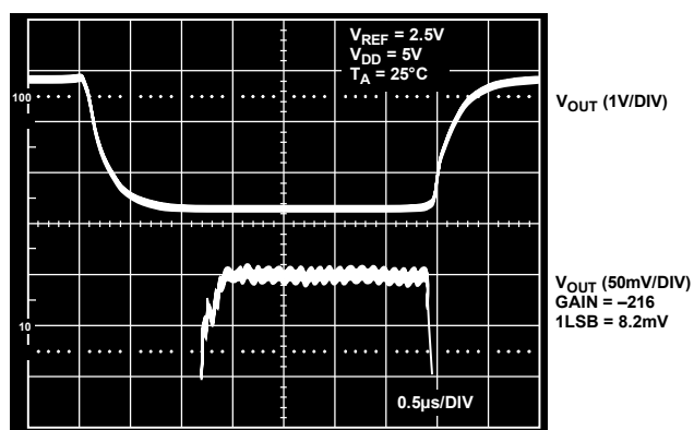
Figure 27. Small Signal Settling Time
