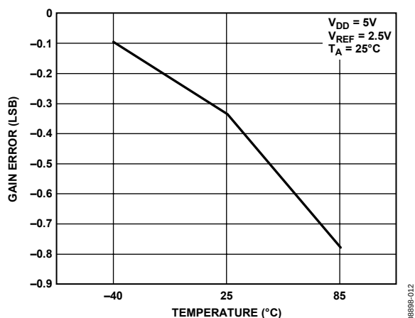
Figure 18. Gain Error vs. Temperature 1
