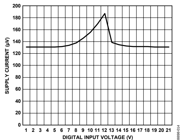
Figure 20. Supply Current vs. Digital Input Voltage
