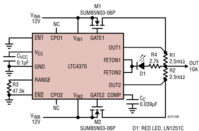
Figure 6. Current Sharing 12V Supplies
