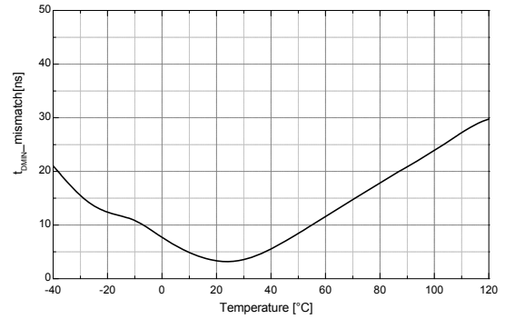
Figure 18. Dead-Time Mismatch vs. Temperature
