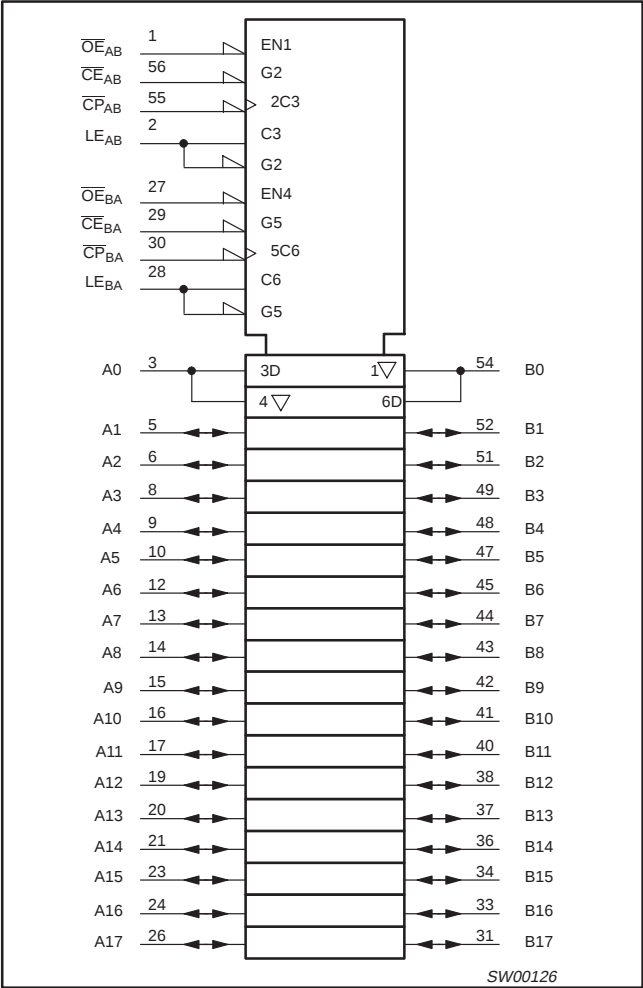
LOGIC SYMBOL (IEEE/IEC)
