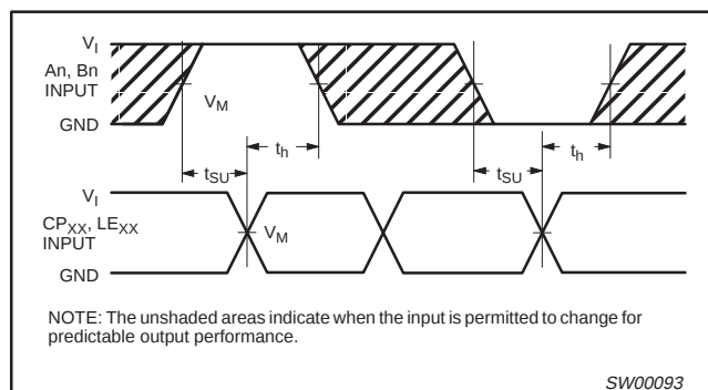
Waveform 4. Data set-up and hold times for the An and Bn inputs to the LE_{AB} , LE_{BA} , \overline{CP}_{AB} and \overline{CP}_{BA} inputs
