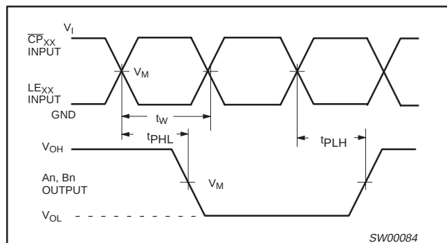
Waveform 2. Latch enable input ( LE_{AB} , LE_{BA} ) and clock pulse input ( \overline{CP}_{AB} , \overline{CP}_{BA} ) to output (An, Bn) propagation delays and latch enable pulse width
