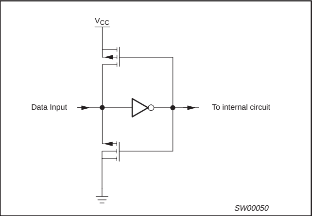
BUSHOLD CIRCUIT
