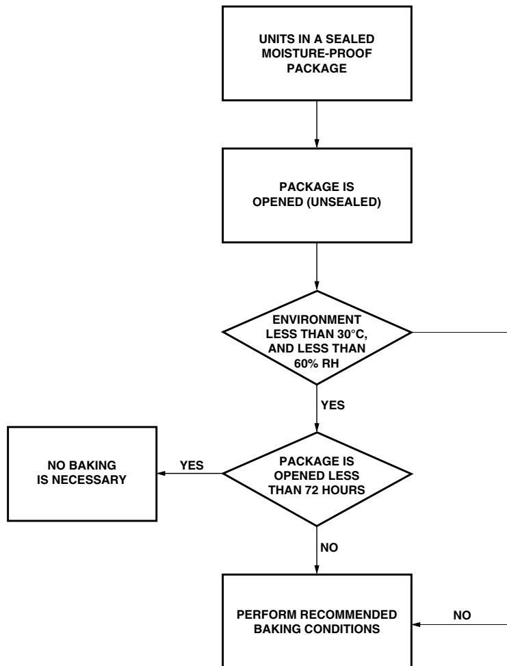
Figure 16. Baking conditions.
