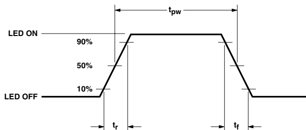
Figure 8. LED optical waveform.
