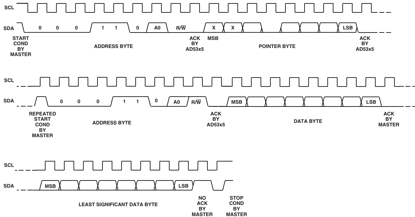
Figure 9. Readback Sequence
