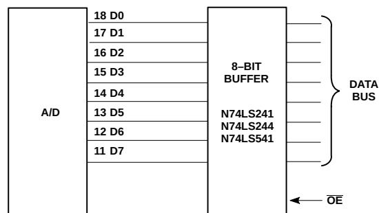
Figure 9. Buffering the A/D Output to Drive High Capacitance Loads and for Driving Off-Board Loads
