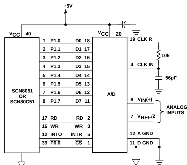
Figure 8. SCN8051 Interfacing
