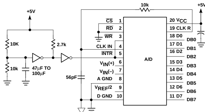
Figure 5. Connection for Continuous Conversion
