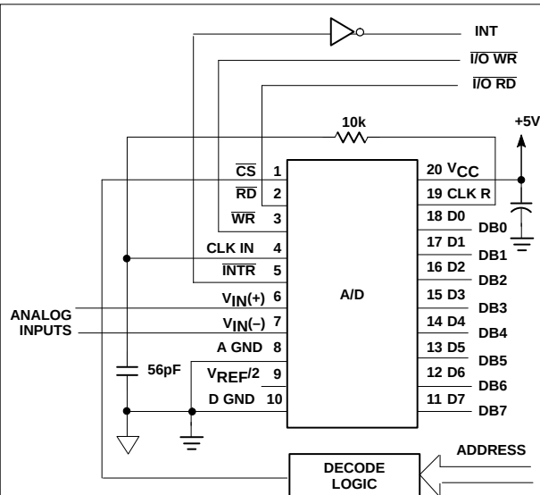
Figure 7. Interfacing to 8080A Microprocessor
