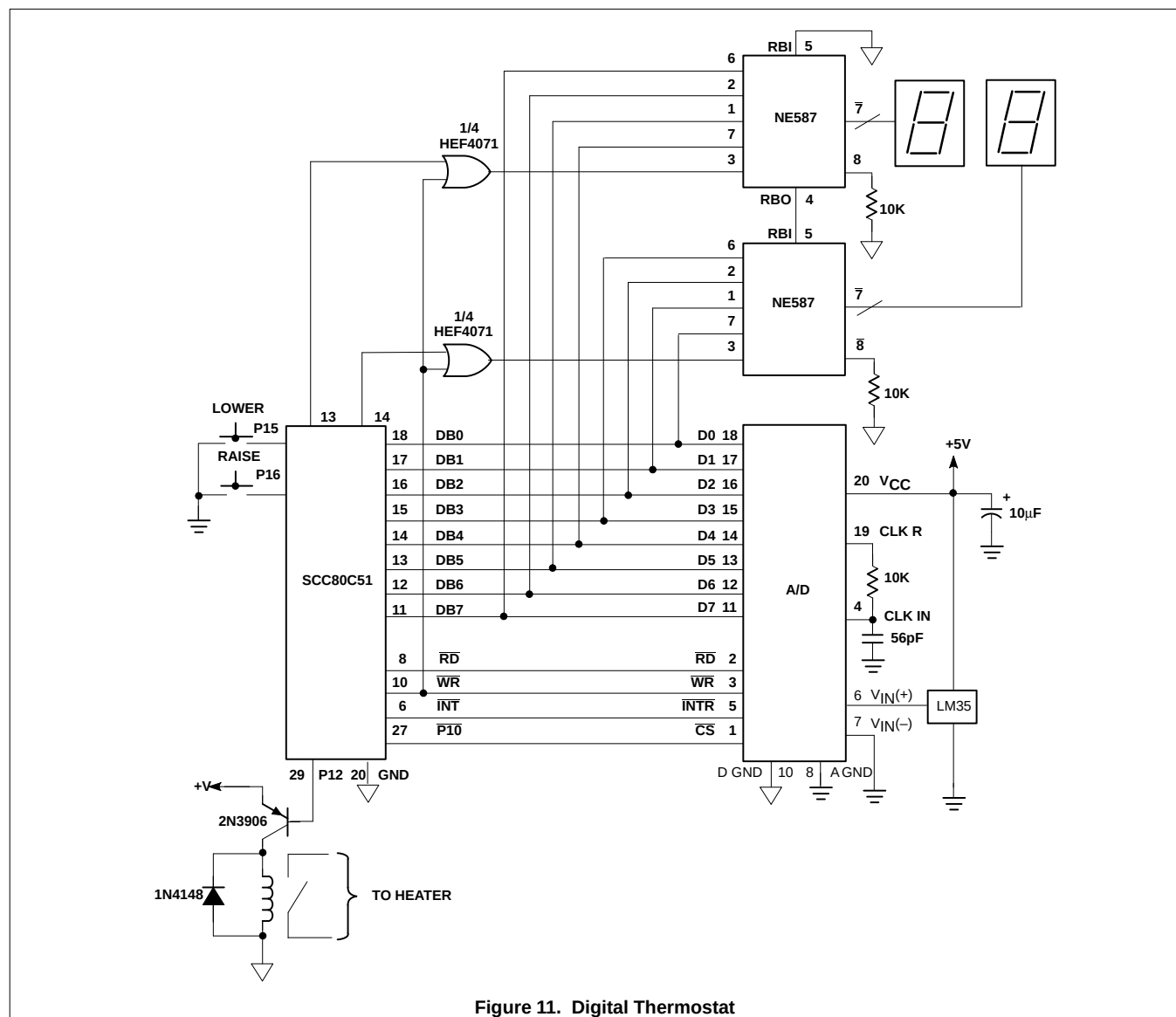
Figure 11. Digital Thermostat
