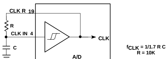
Figure 5. Connection for Continuous Conversion
