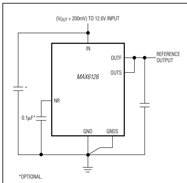
Figure 1. Noise-Reduction Capacitor
