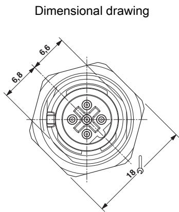
M12 flush-type connector
