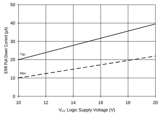
Figure 33B. ERR Pull-Down Current vs. Voltage
