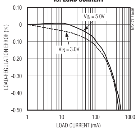
LDO OUTPUT LOAD REGULATION vs. LOAD CURRENT
