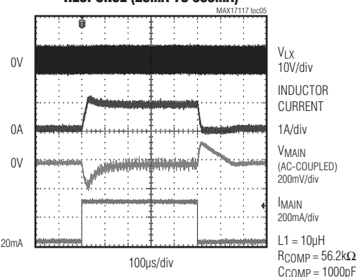
STEP-UP REGULATOR LOAD-TRANSIENT RESPONSE (20mA TO 300mA)
