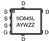
DFN5 CASE 488AA DFNW5 CASE 507BA
