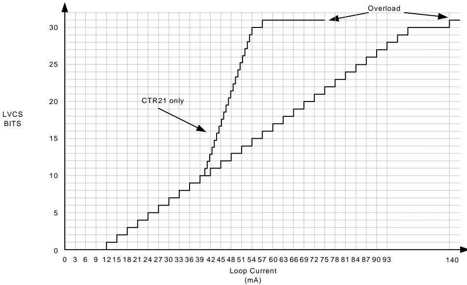
Figure 7. Loop Current
