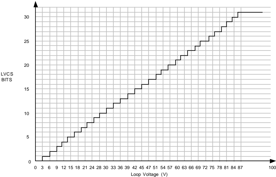
Figure 6. Loop Voltage
