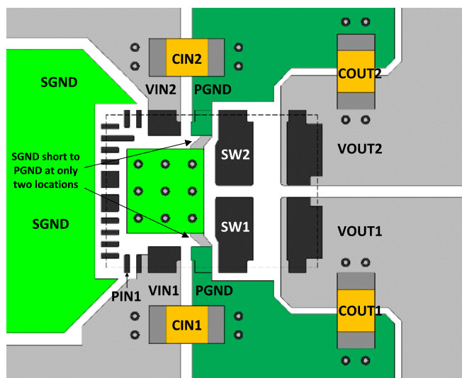
FIGURE 31. RECOMMENDED LAYOUT
