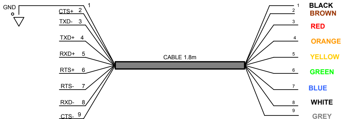
Figure 5.1 USB-RS422-WE Connections
