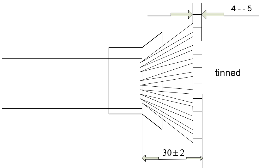
Figure 5.2 USB-RS422-WE Mechanical Details (dimensions in mm)
