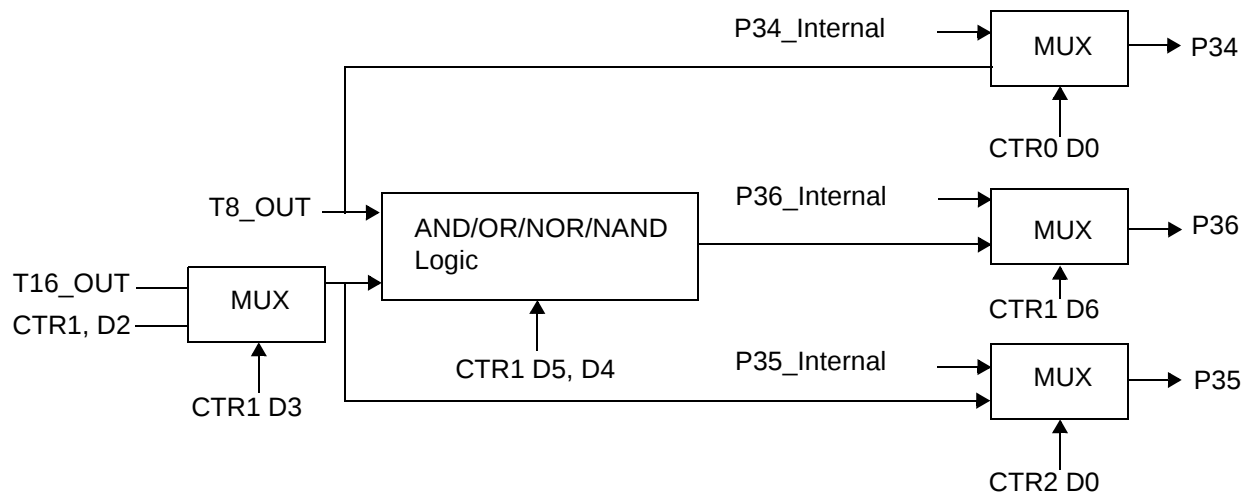
Figure 24. Output Circuit
