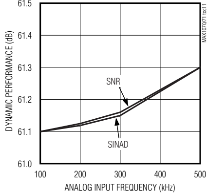
DYNAMIC PERFORMANCE vs. INPUT FREQUENCY (MAX1071)
