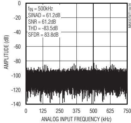
FFT PLOT (MAX1070)
