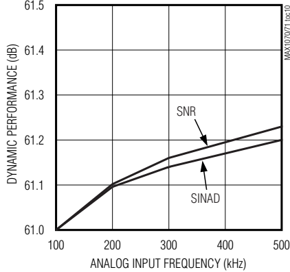
DYNAMIC PERFORMANCE vs. INPUT FREQUENCY (MAX1070)
