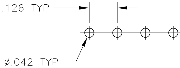
RECOMMENDED HOLE LAYOUT
