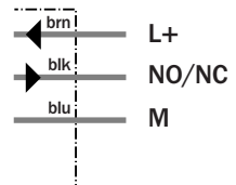
3 x 0.5 mm²
