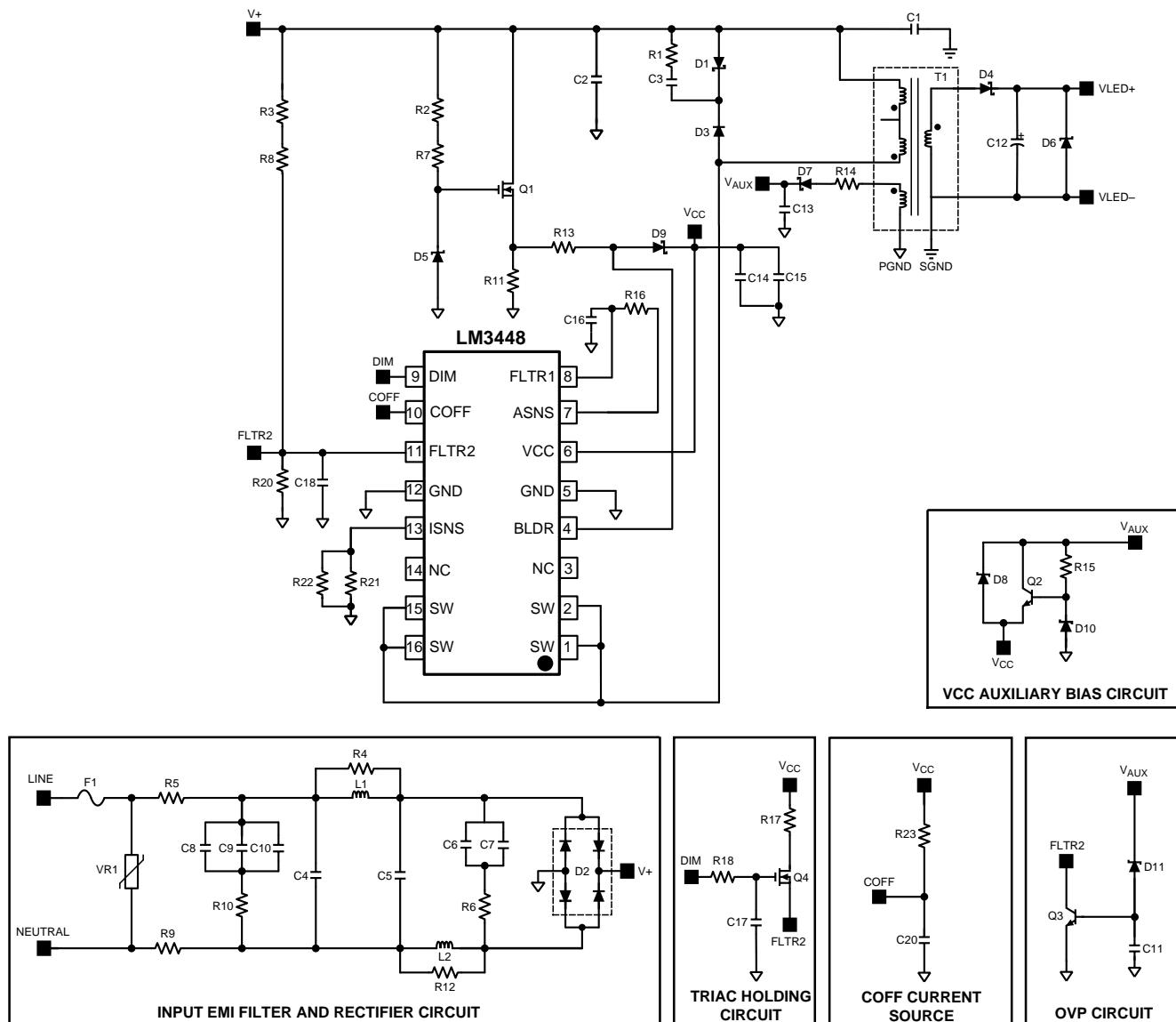
Figure 42. DESIGN #4 Circuit
