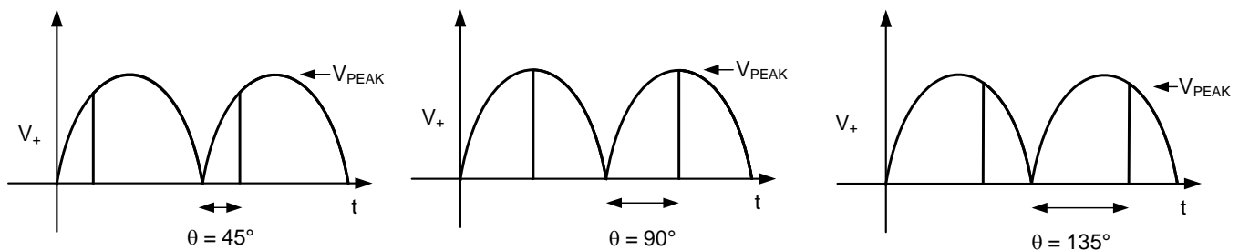
Figure 37. V_{\text{BUCK}} Waveforms with Various TRIAC Firing Angles
