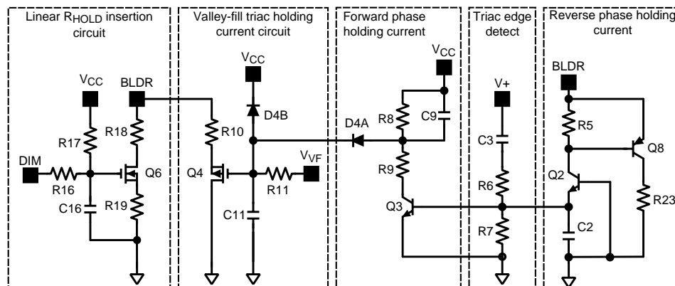
Figure 39. DESIGN #1 Circuit
