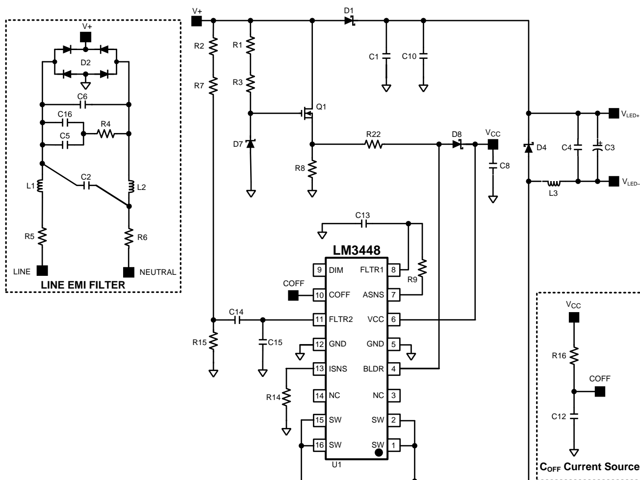
Figure 40. DESIGN #2 Circuit
