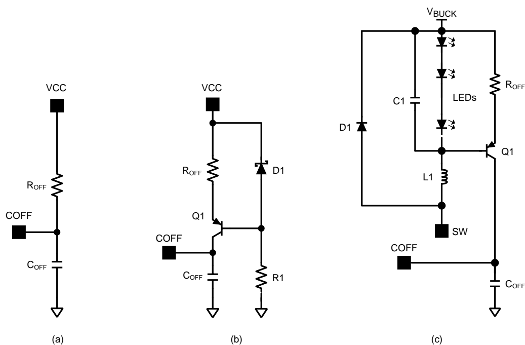
Figure 32. COFF Current Source Circuits
