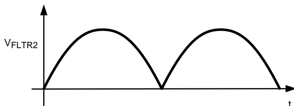
Figure 26. FLTR2 Waveform with No Dimmer
