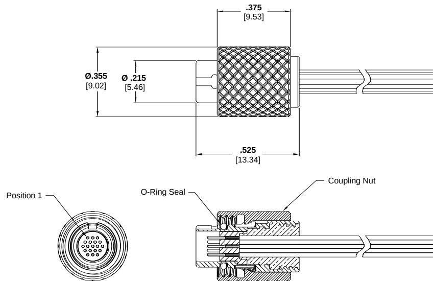
19 Position Drawing Number 1589064
