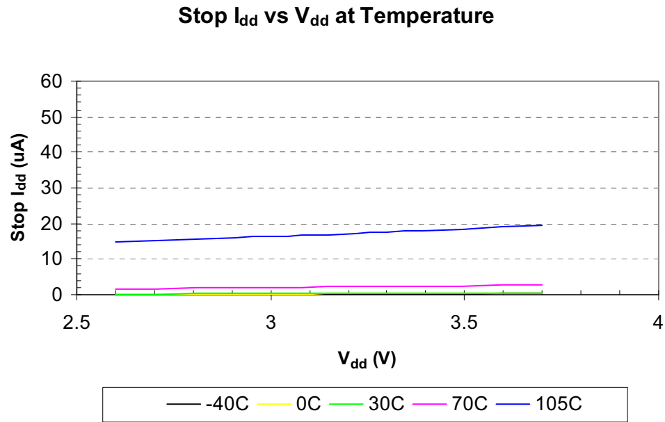
Figure 63. Stop Mode Current Versus V_{DD}
