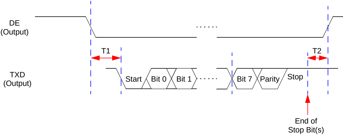
Figure 69. UART Timing without \overline{\text{CTS}}
