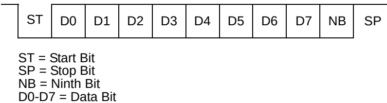
Figure 55. 9-Bit Mode
