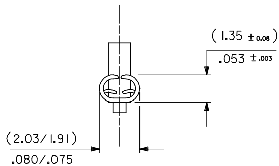
CRIMP DETAIL
