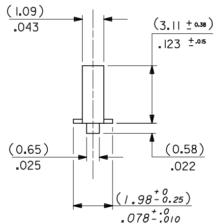
CRIMP DETAIL
