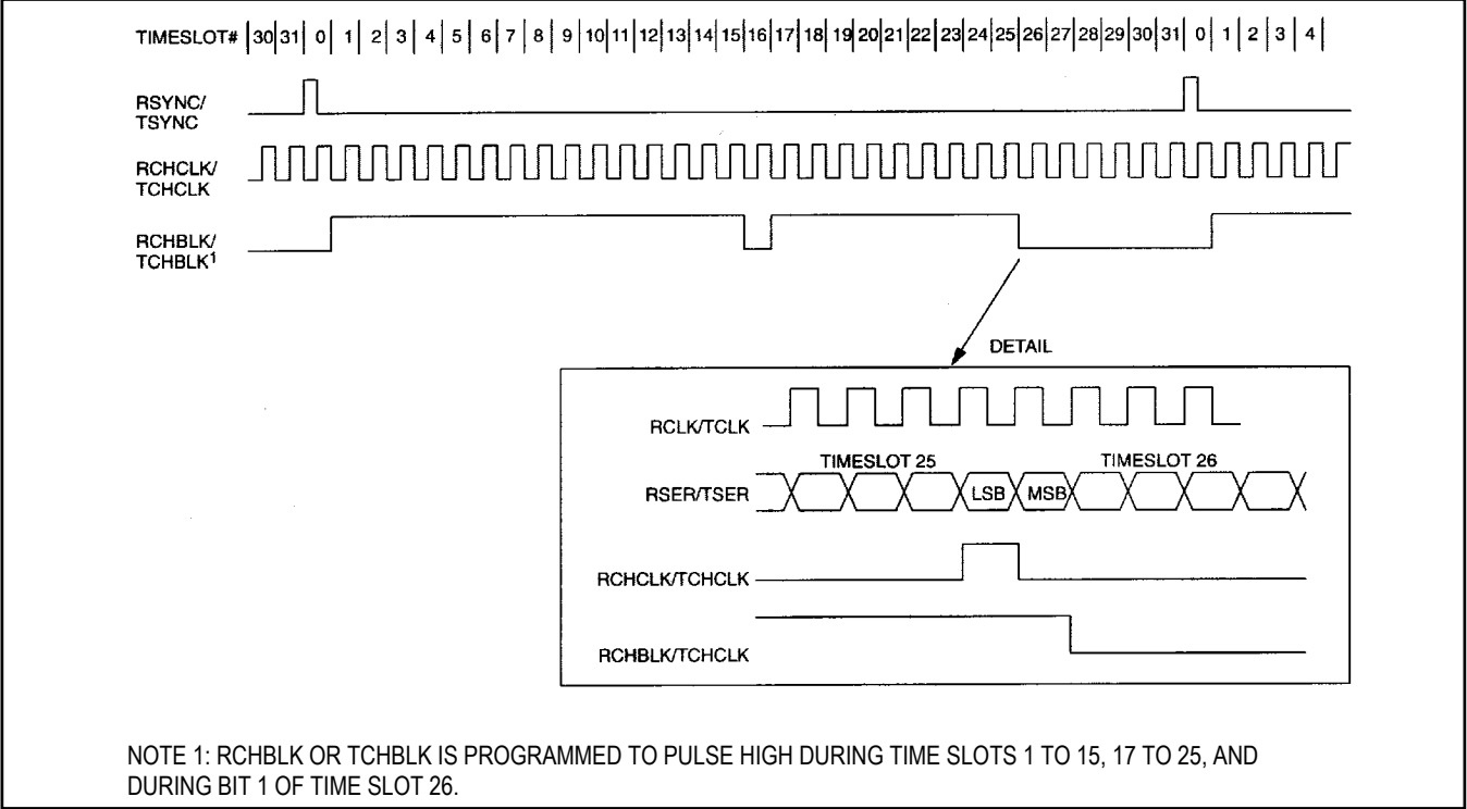
Figure 14-7. G.802 Timing
