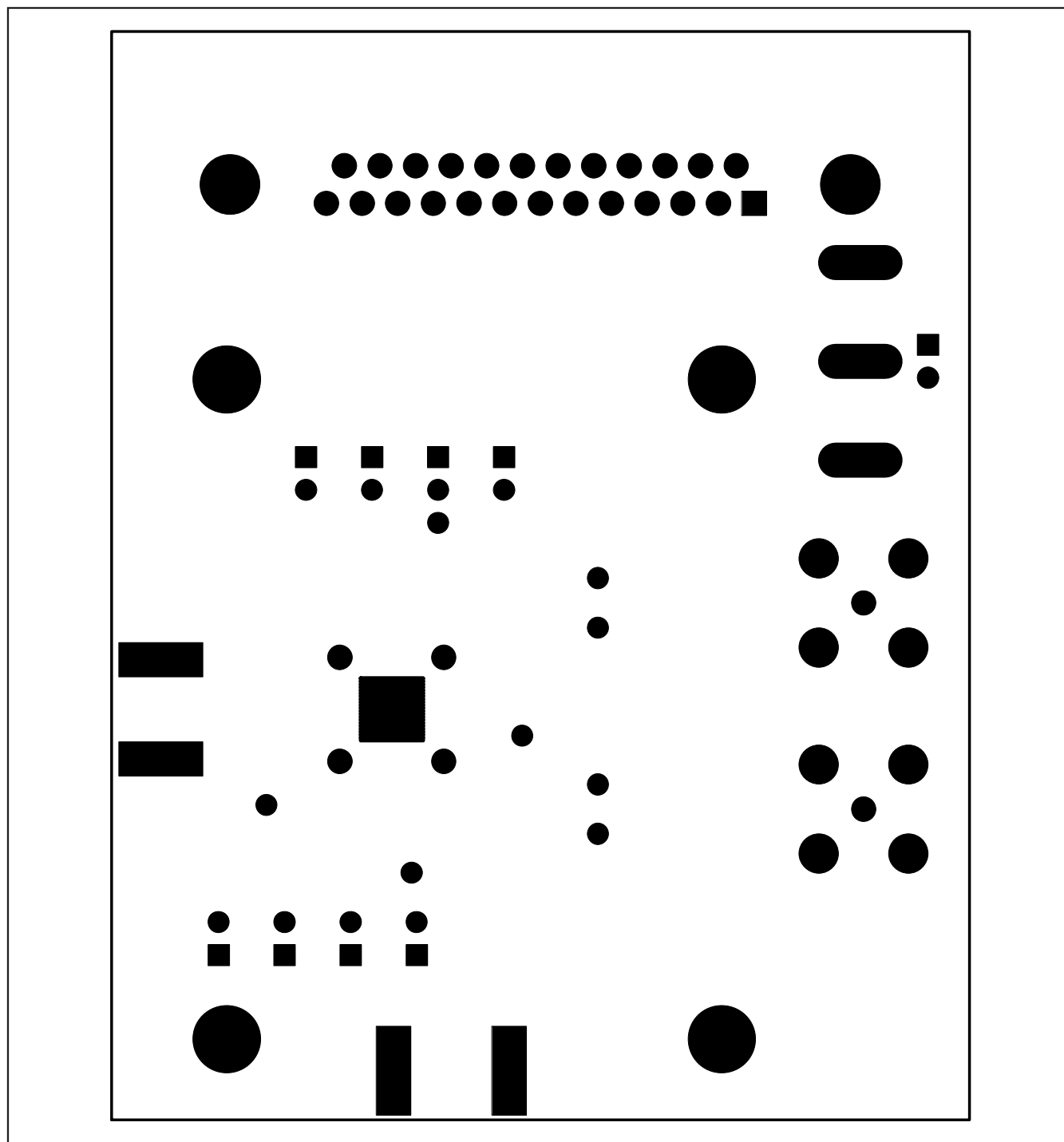
Figure 6. MAX2117 EV Kit PCB Layout—Bottom Soldermask
