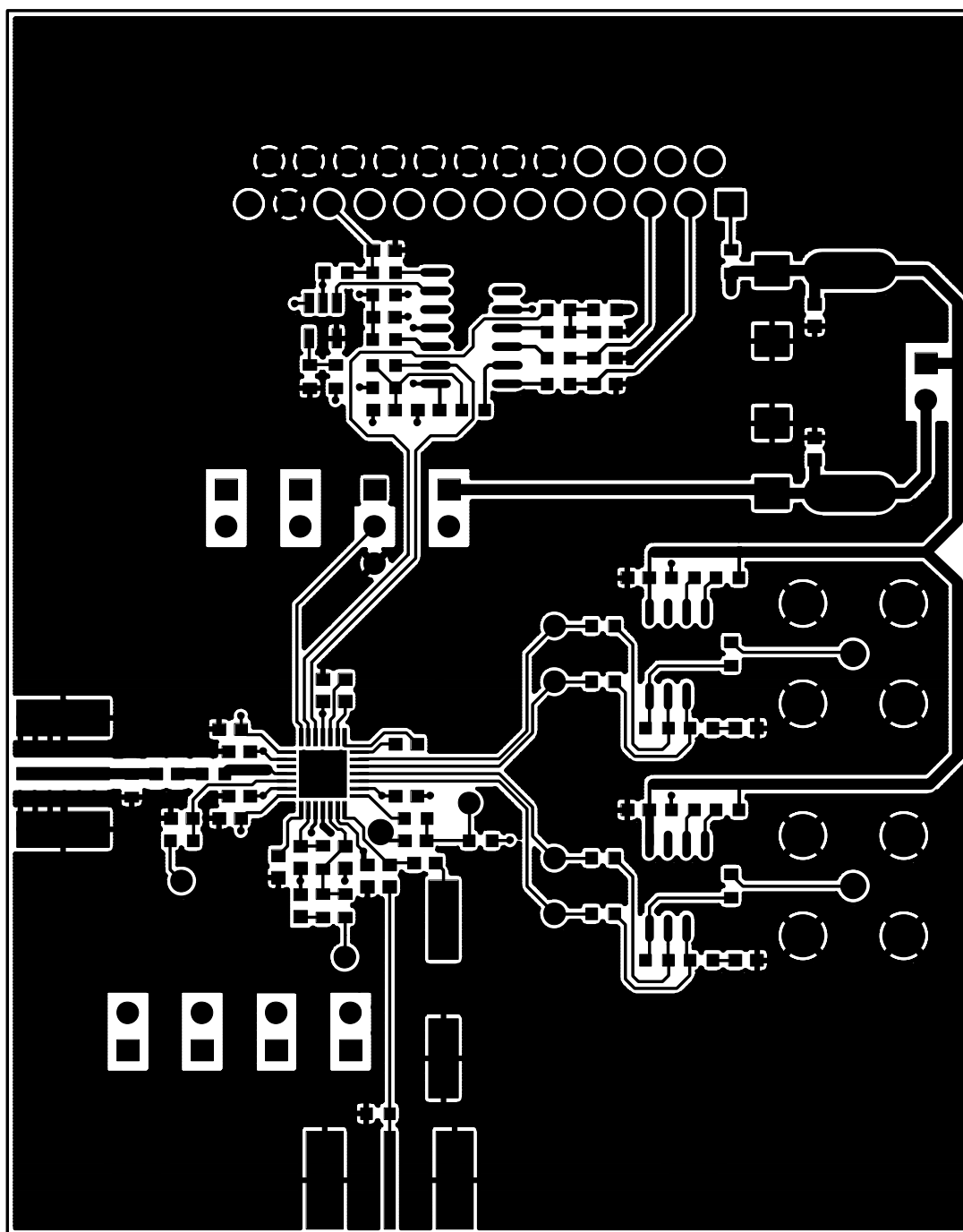
Figure 3. MAX2117 EV Kit PCB Layout—Top
