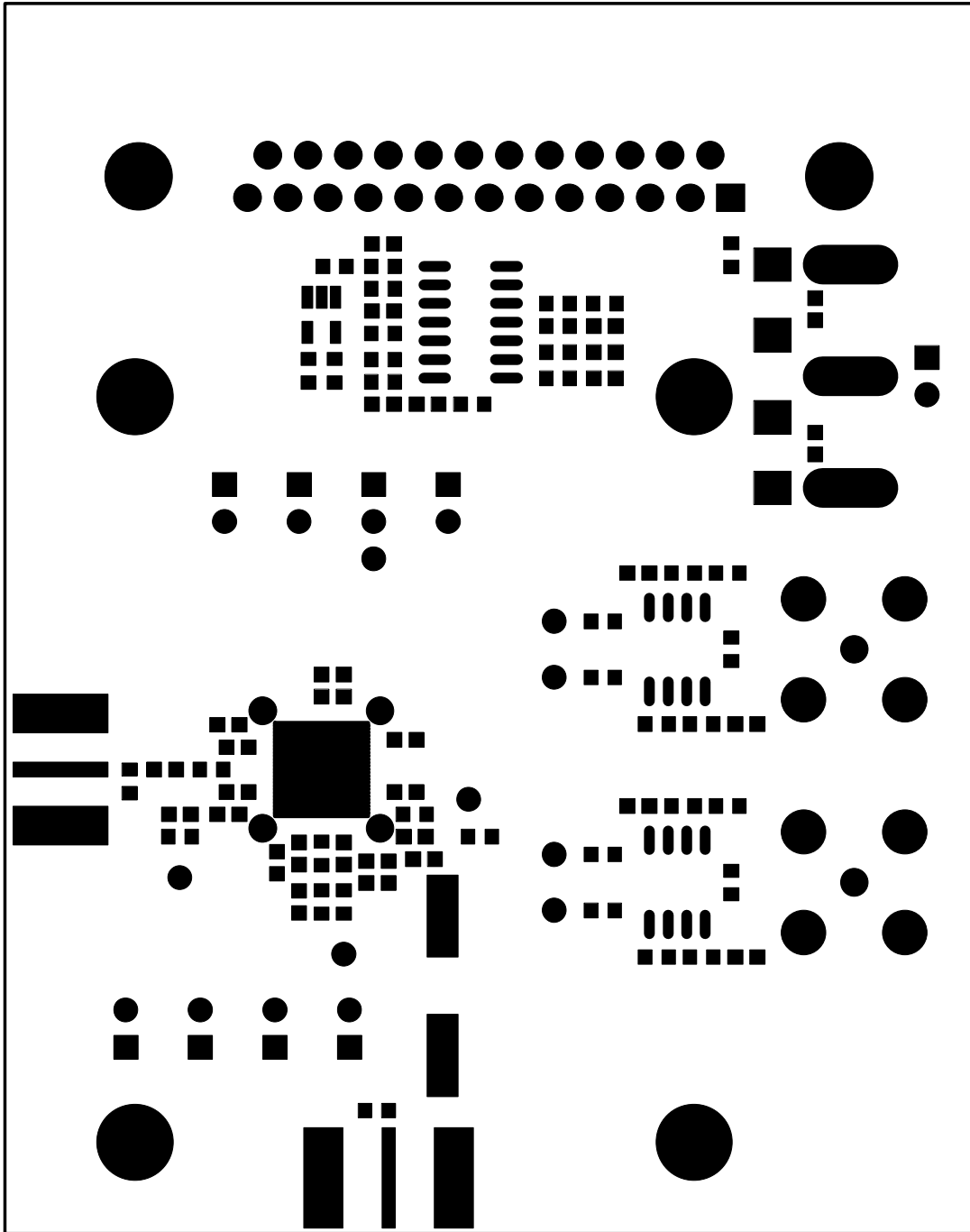
Figure 5. MAX2117 EV Kit PCB Layout—Top Soldermask
