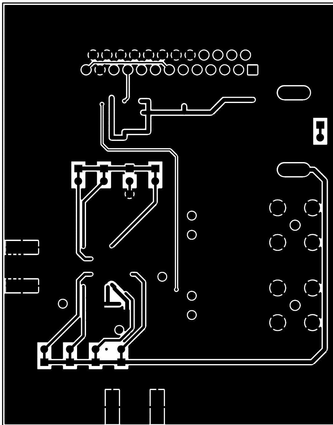
Figure 4. MAX2117 EV Kit PCB Layout—Bottom
