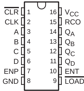
SN54HC161 . . . J OR W PACKAGE SN74HC161 . . . D, N, NS, OR PW PACKAGE (TOP VIEW)
