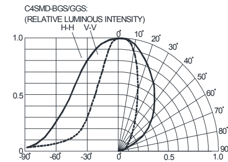
FIG.6a BLUE&GREEN FAR FIELD PATTERN
