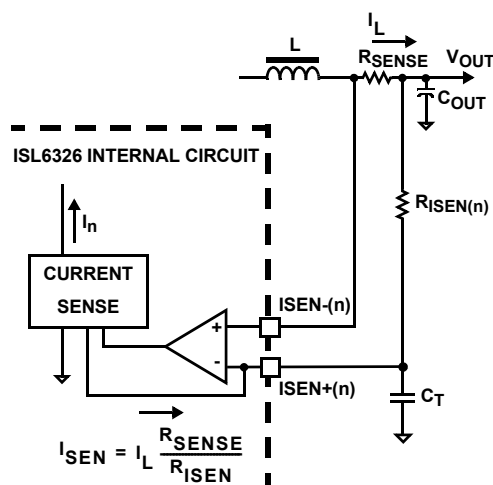
FIGURE 4. SENSE RESISTOR IN SERIES WITH INDUCTORS
