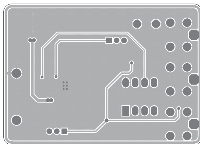
Figure 6: AAT3171 Evaluation Board Bottom Side Layout.
