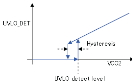
Figure 3. UVLO Hysteresis
