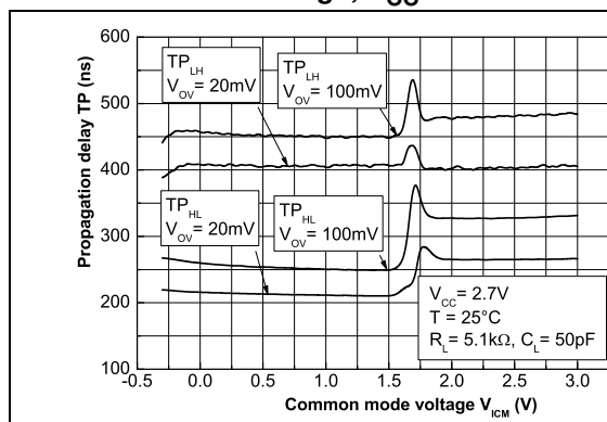
Figure 20. Propagation delay versus common mode voltage, V_{CC} = 2.7\text{ V}
