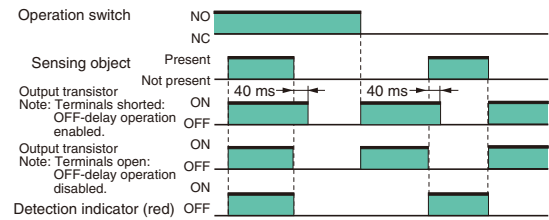
Timing Chart
