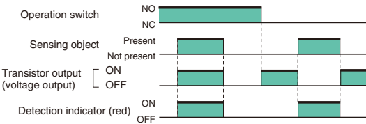
Timing Chart
