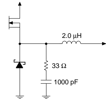
Figure 18. Filter Components
