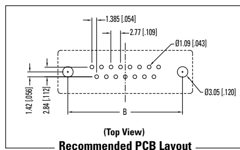
(Top View) Recommended PCB Layout
