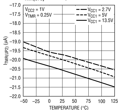
I_{TMR(UP2)} vs Temperature
