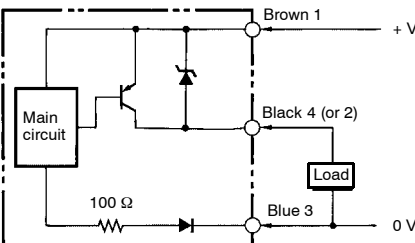
E2E2-X□B□ DC 3-wire Models
