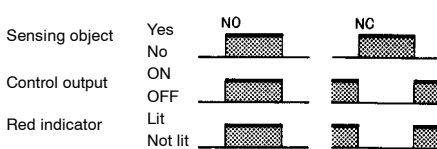
NPN/PNP Open Collector Output
