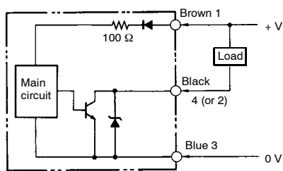
E2E2-X□C□ DC 3-wire Models
