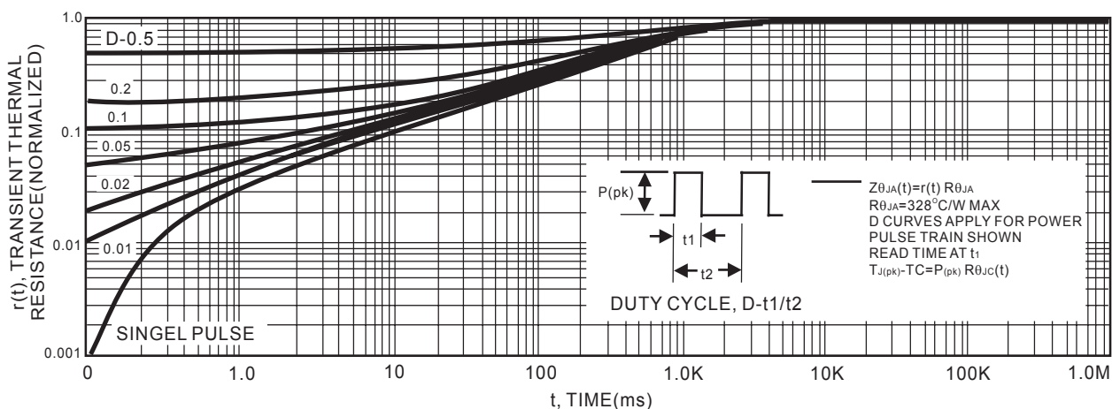
Figure 7. Thermal Response
