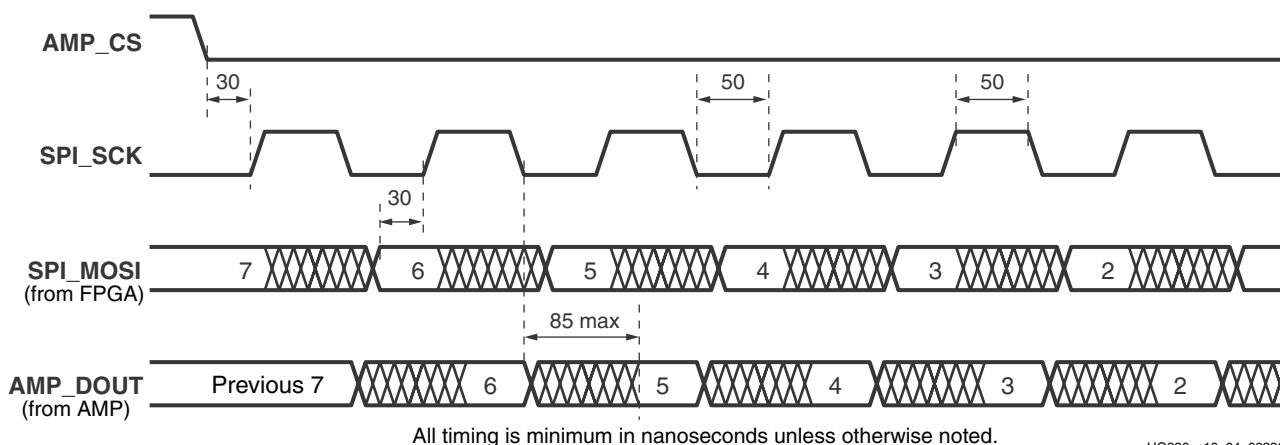
Figure 10-4: SPI Timing When Communicating with Amplifier
