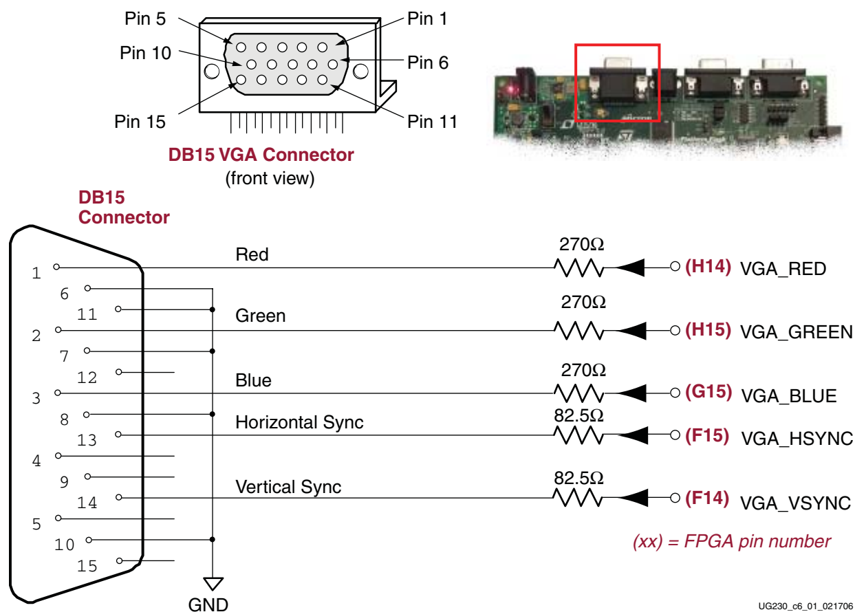
Figure 6-1: VGA Connections from Spartan-3E Starter Kit Board
