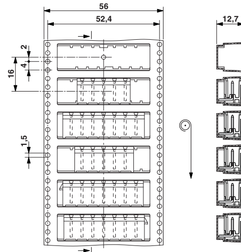
Dimensioned drawing
