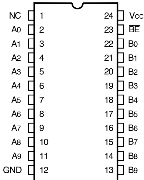
QSOPTOP VIEW
