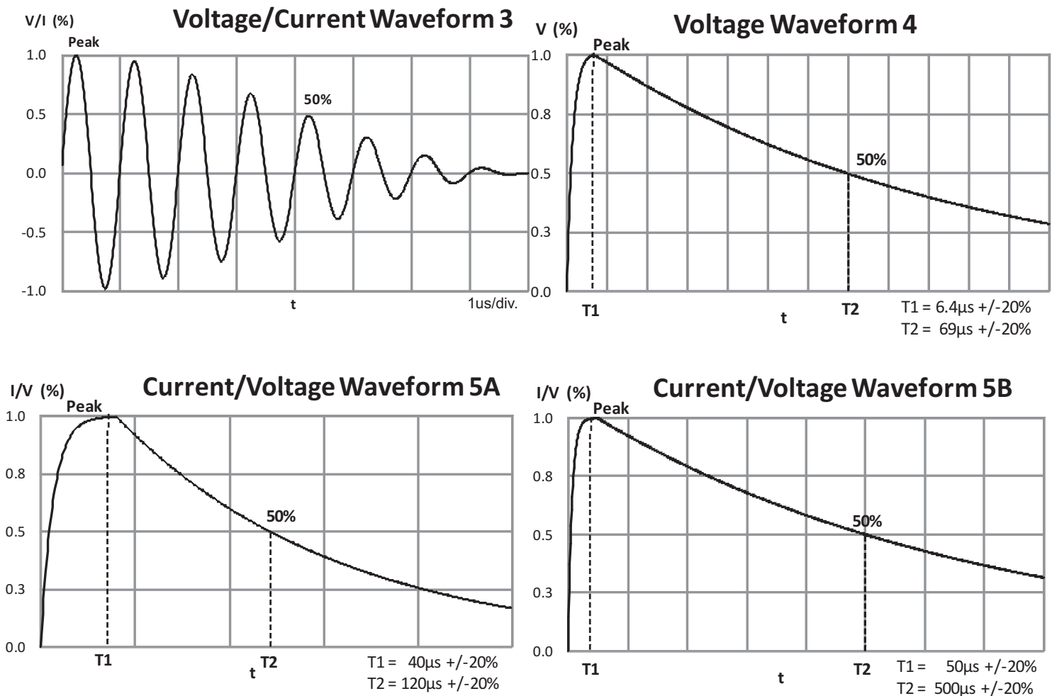
Figure 10. Lightning Waveforms
