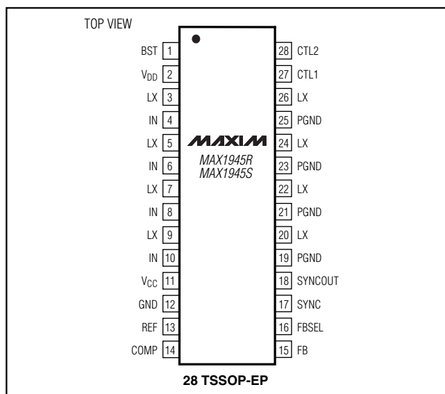
Pin Configuration
