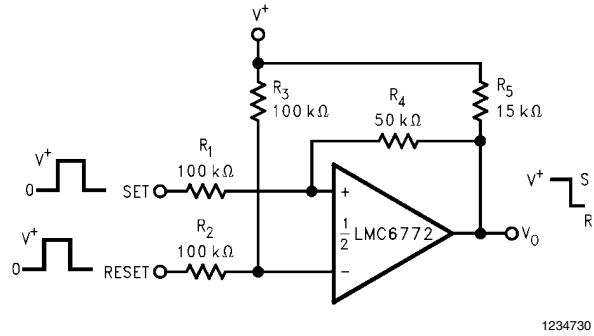
FIGURE 6. Bi-Stable Multivibrator
