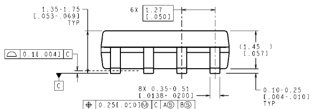
8-Pin SOIC NS Package Number M08A
