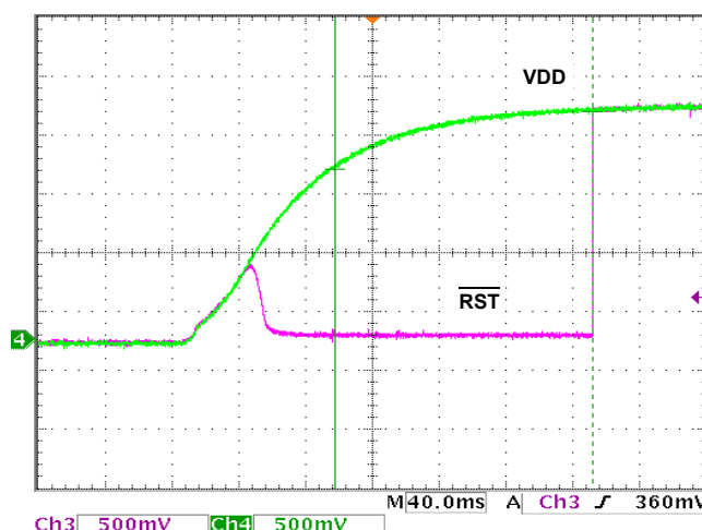
FIGURE 4. ISL88002 \overline{\text{RST}} t_{POR} ~155ms, R_{PU} = 5\text{ k}\Omega
